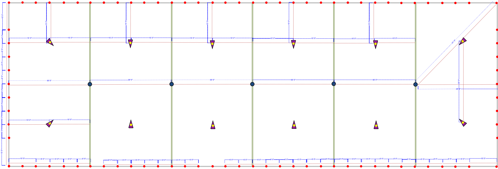
60' x 180' Pole Tent - Pole Placements
